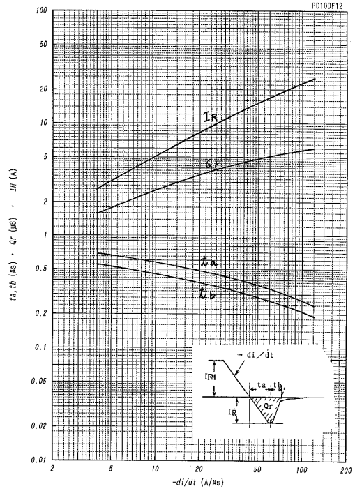
逆回復特性(代表例) REVERSE RECOVERY CHARACTERISTICS (TYP) Tj=150°C, IFR=100 A
