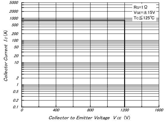
Fig. 10 Reverse Bias Safe Operating Area (Typical)
