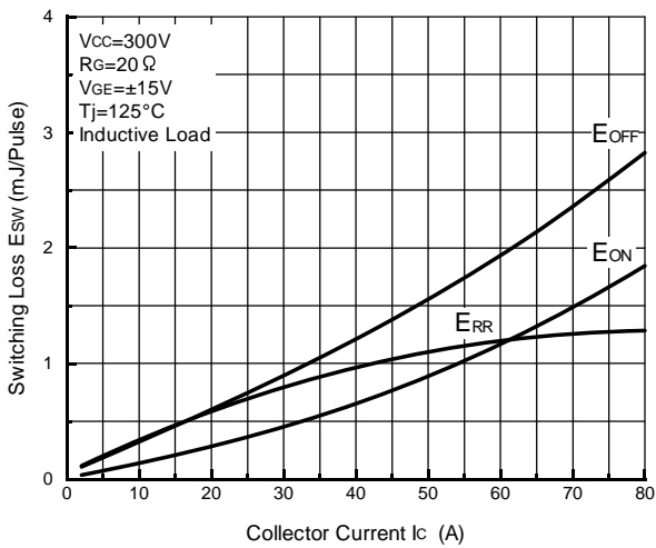
Fig.11- Collector Current vs. Switching Loss
